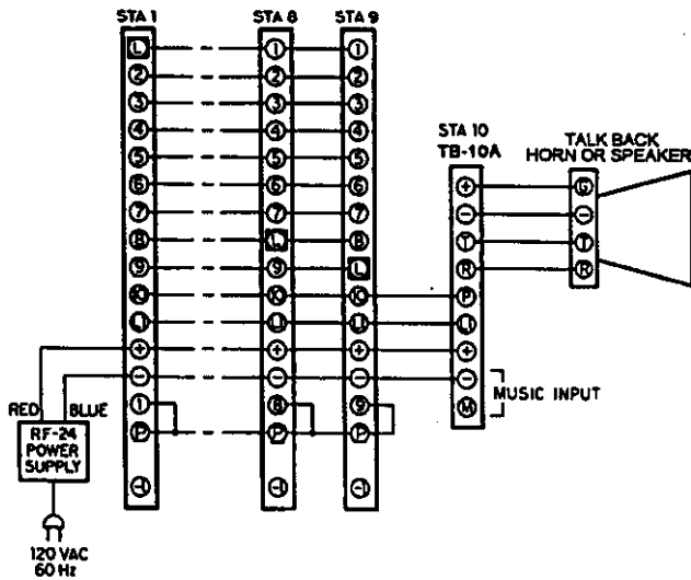
Figure 3. Using TB10A Page Adaptor for Additional Page Channel with Talkback.
