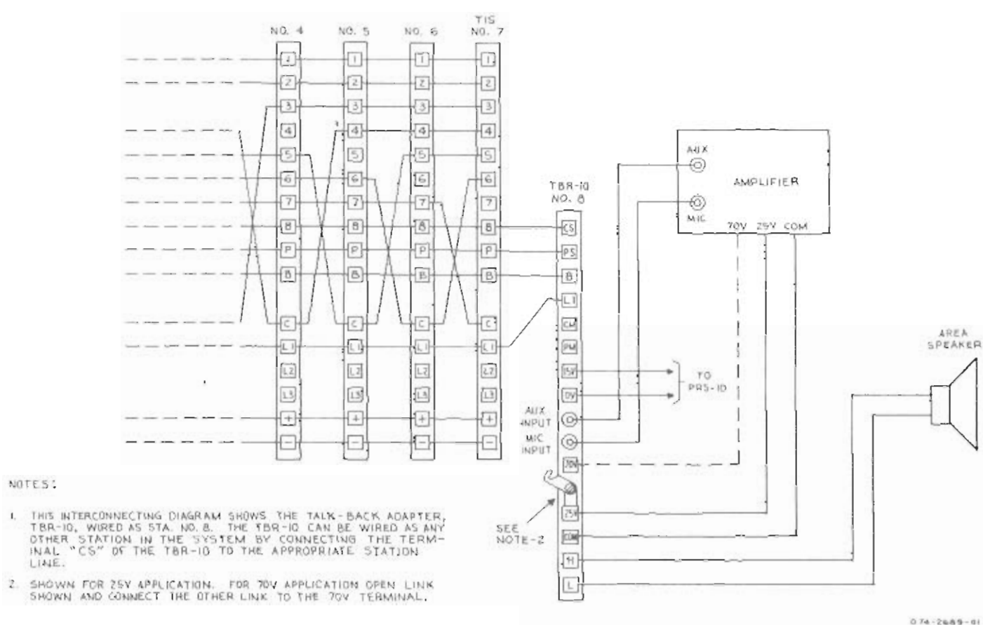
Figure 9 — Talk-Back Adapter TBR-10 — Connection Diagram
