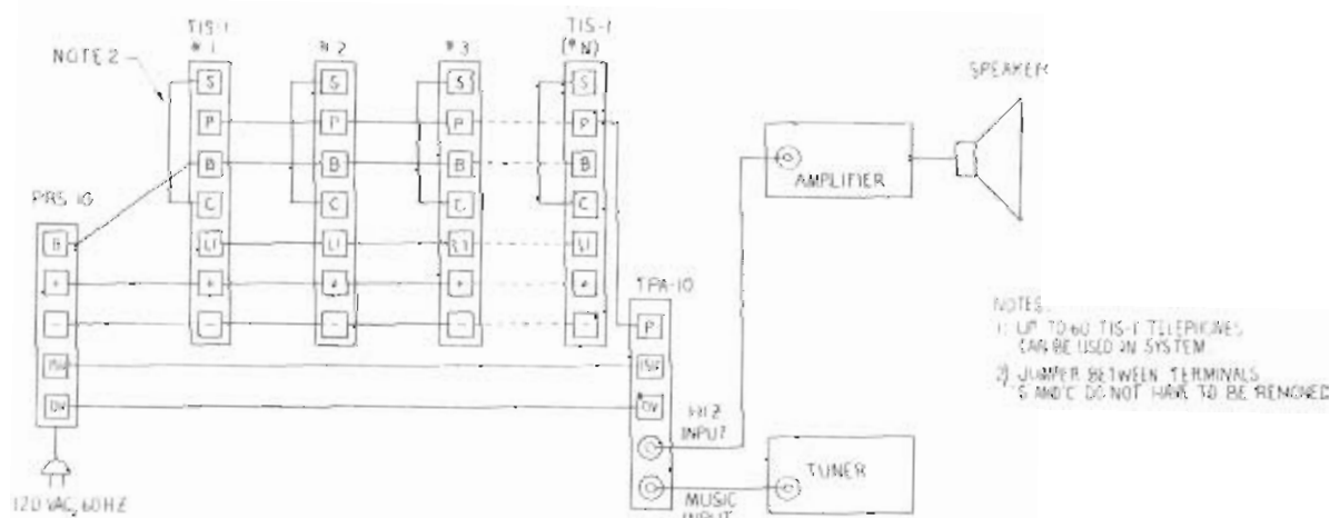
Figure 5 — Multiple TIS-1 with TPA-10 Page Adapter
