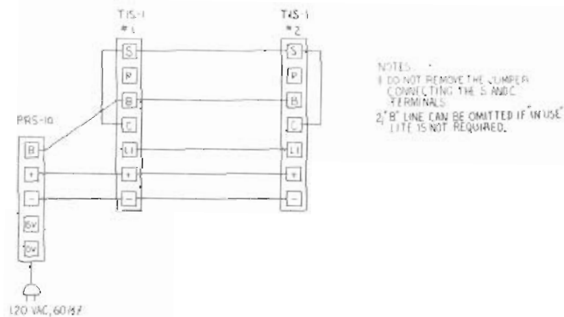
Figure 4 — Two TIS-1 Stations Ring and Talk -- Interconnection Diagram
