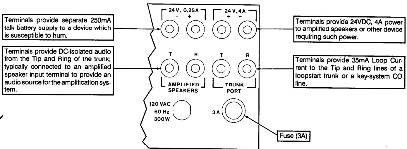
Figure 1 - PRS-624DA Rear Panel Illustration
