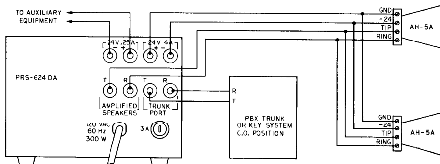
Figure 2 - Typical Installation Wiring
