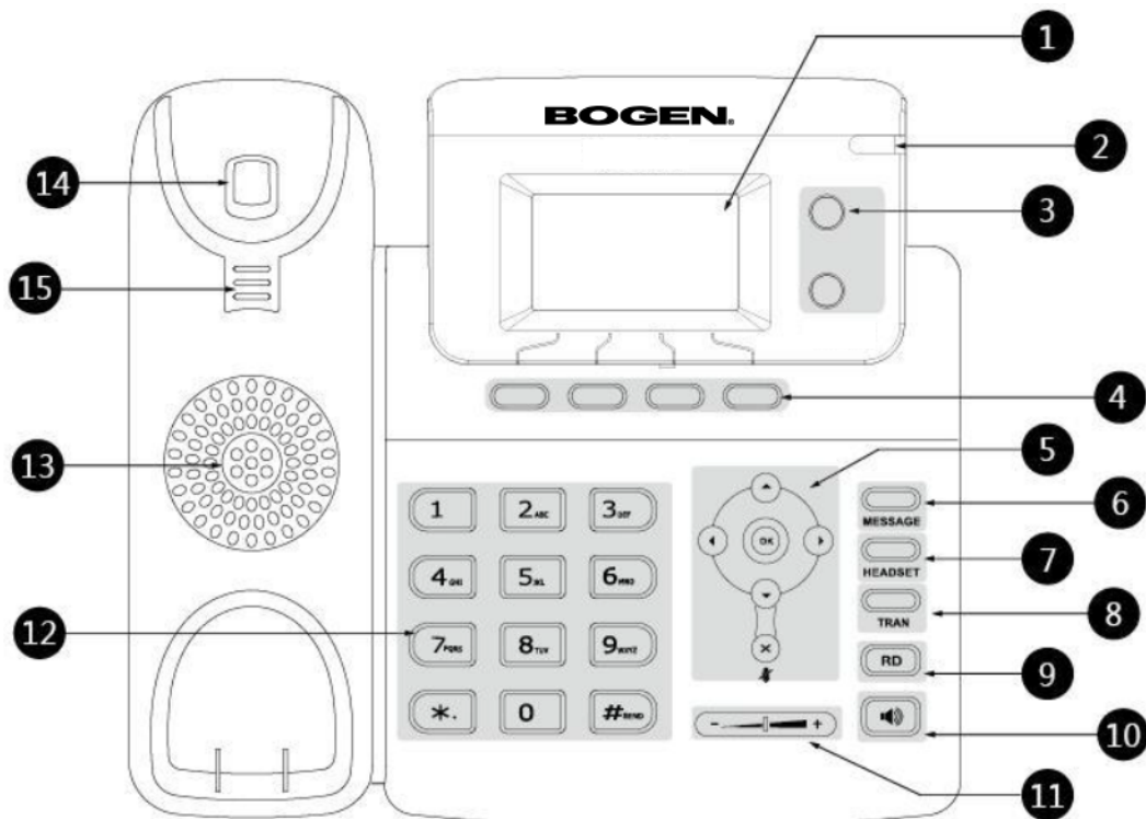
Figure 1-1, Hardware Components
