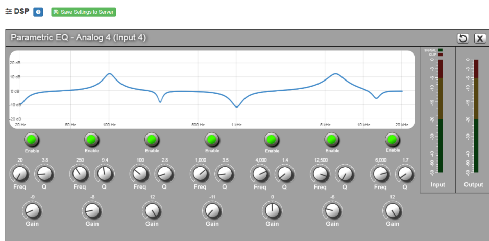
Figure 13, Parametric Equalizer Settings
