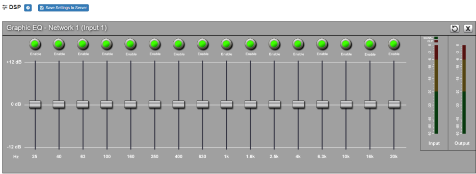
Figure 9, Graphic EQ Settings
