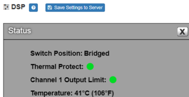
Figure 20, Status When Channels 1 and 2 Are Bridged
