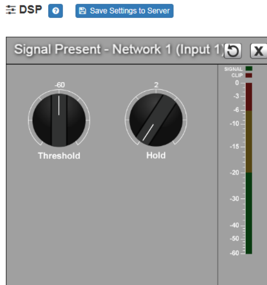
Figure 19, Signal Present Parameters
