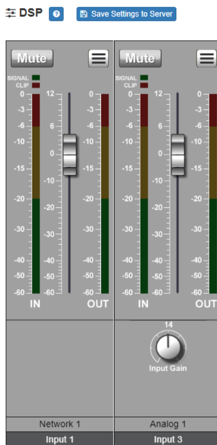
Figure 8, DSP for Single Channel Bridged Mode
