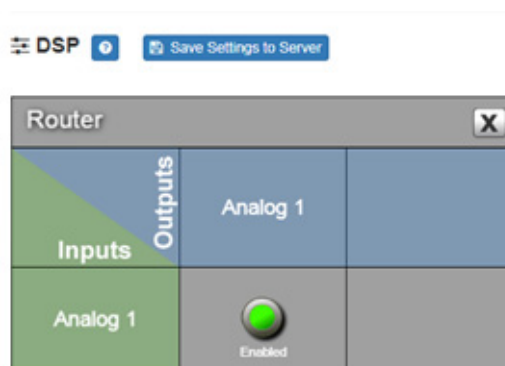
Figure 16, Router for Single Channel Bridged Mode
