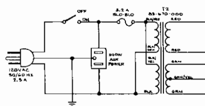
Figure 2 - 120 V. Line Wiring.
