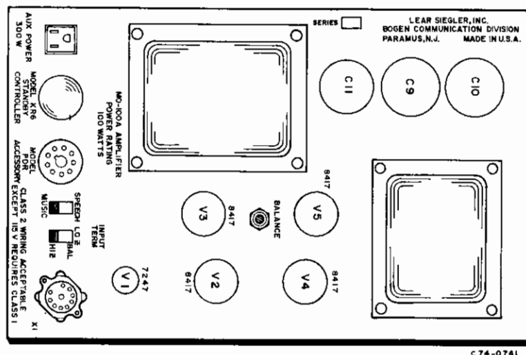
Figure 5 - Top View of Chassis
