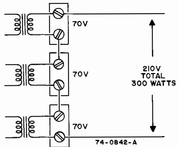
Figure 3 - Series Hookup of 70-Volt Outputs
