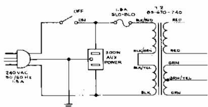
Figure 1 - 240 V. Line Wiring.
