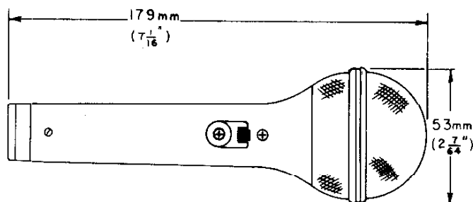
FIGURE 3: DIMENSIONS
