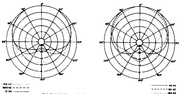
FIGURE 2: POLAR RESPONSE
