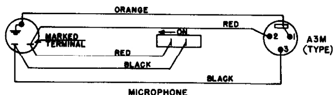
FIGURE 4: WIRING DIAGRAM
