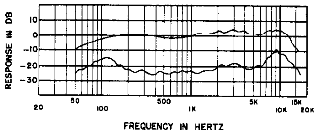
FIGURE 1: FREQUENCY RESPONSE
