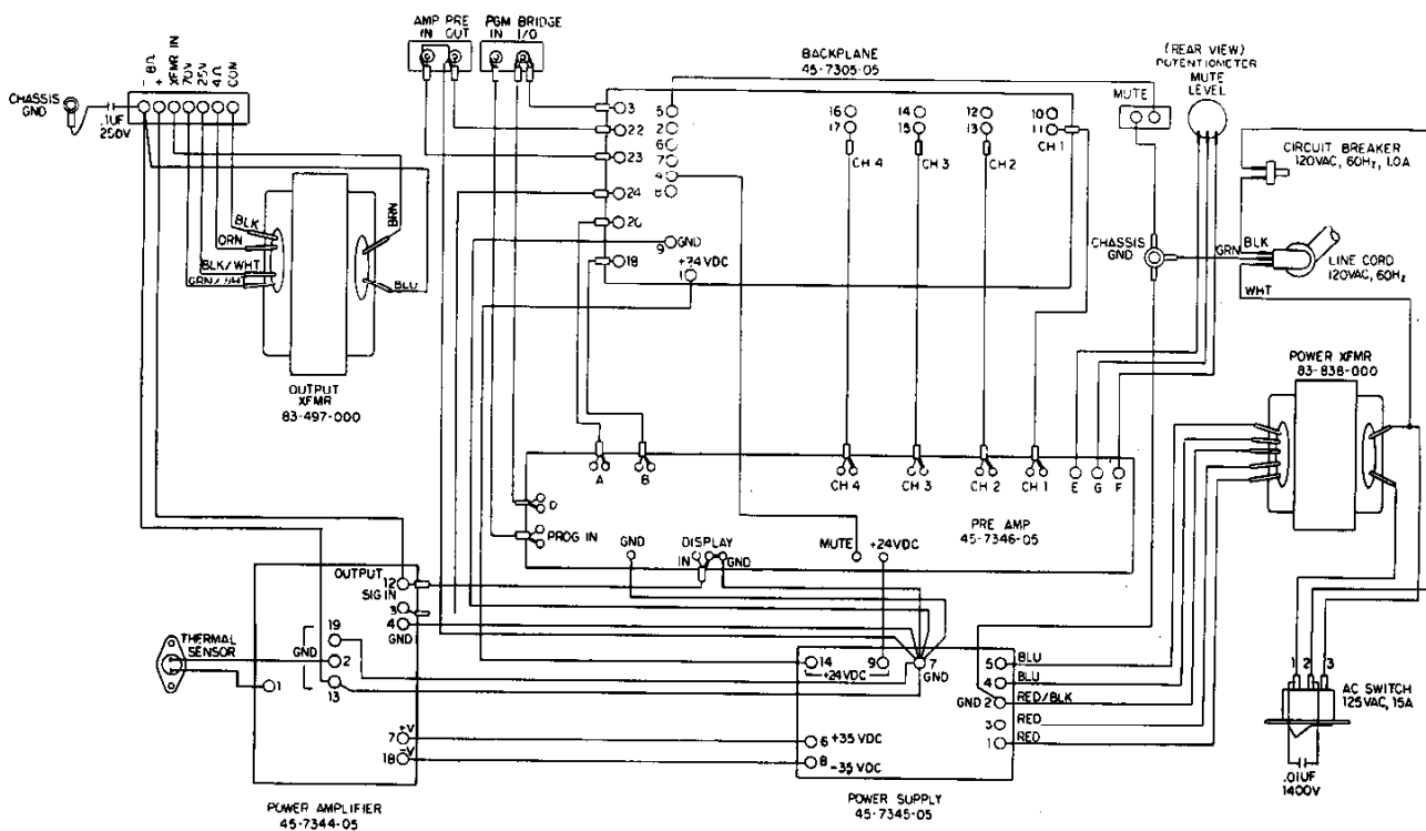
DMA-20 Wiring Diagram
