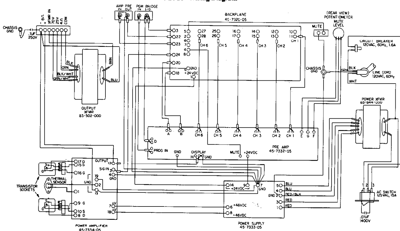
DMA-40 Wiring Diagram
