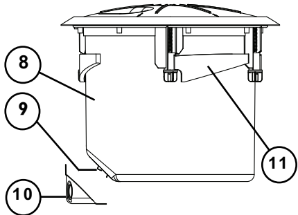
Side Drawing
