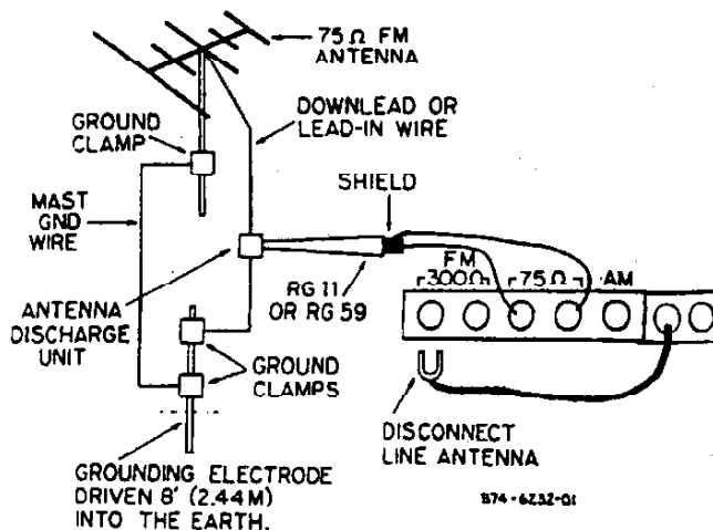
Figure 3 - Connecting Outdoor FM Antenna, 75 Ohm System
