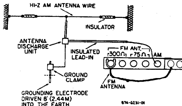
Figure 1 - Connecting Outdoor AM and FM Line Antenna.
