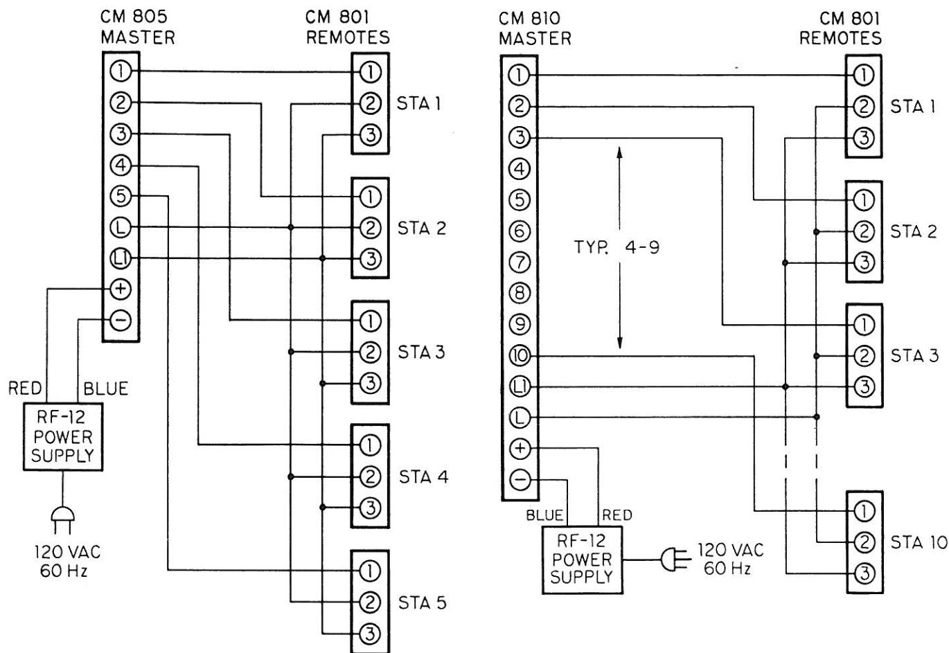
Figure 5—Single Master/Multiple Remote Connection Diagram
