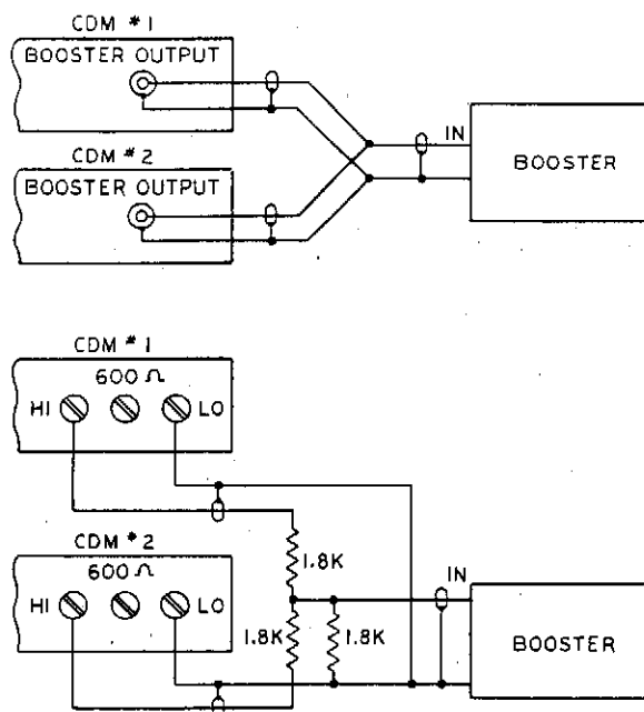
Figure 2 - Bridging options
