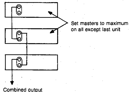
Figure 5 — Series-connected outputs
