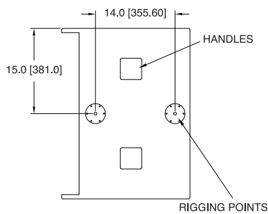
SIDE VIEW (WITHOUT GRILLE)
