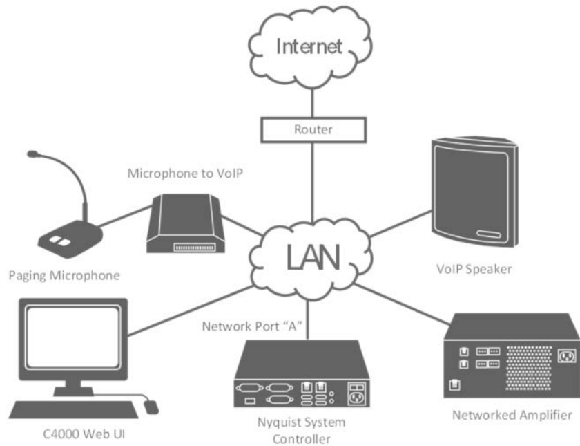
Figure 1. Port A-Only Configuration
