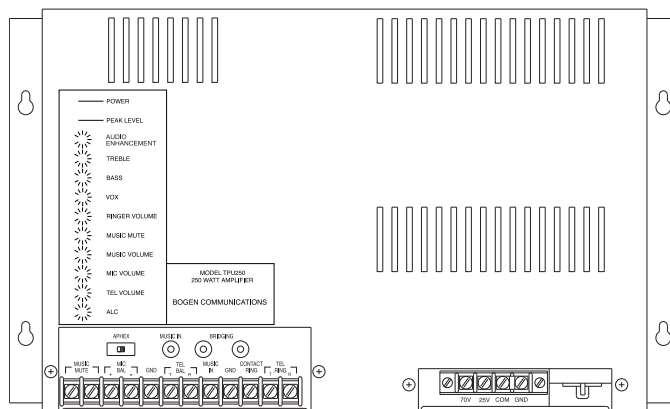
Figure 1a: TPU250 Telephone Paging Amplifier
