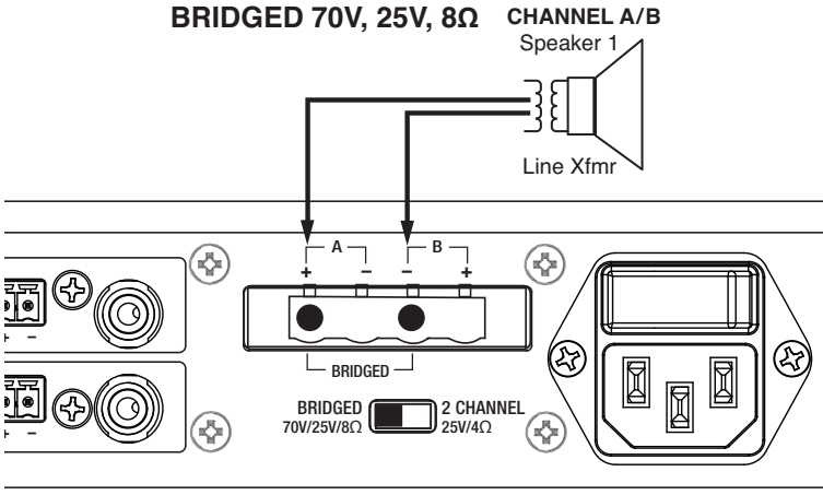
(Figure 1) Bridged Wiring
